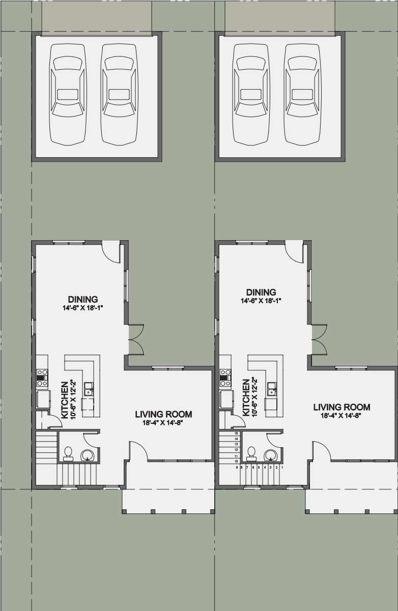
Ground Floor
