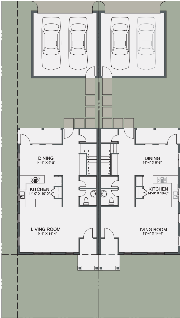
Plan H2- Ground Floor
