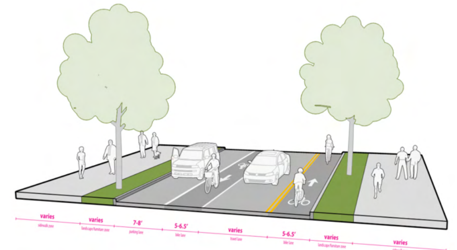
Figure 4-13. Example Cross Section with Contra-flow Bicycle Lanes.
