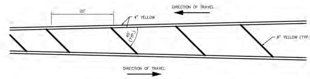
CENTER GORE AREA - PAVEMENT MARKINGS
