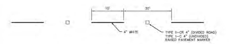
SKIP LANE LINE - PAVEMENT MARKING
