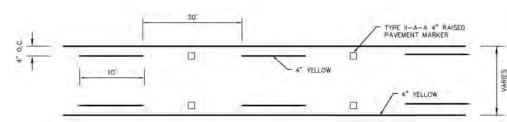
TWO-WAY LEFT TURN LANE - PAVEMENT MARKINGS
