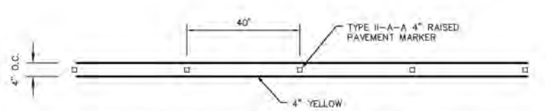
DOUBLE YELLOW LINE - PAVEMENT MARKING
