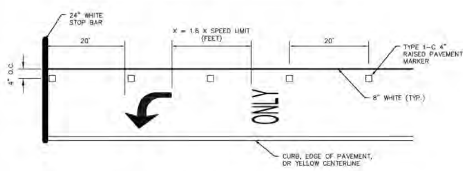
TURN BAY LANE LINE - PAVEMENT MARKERS
