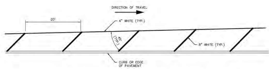
CROSS HATCHING FOR MERGING/SHIFTING - PAVEMENT MARKINGS
