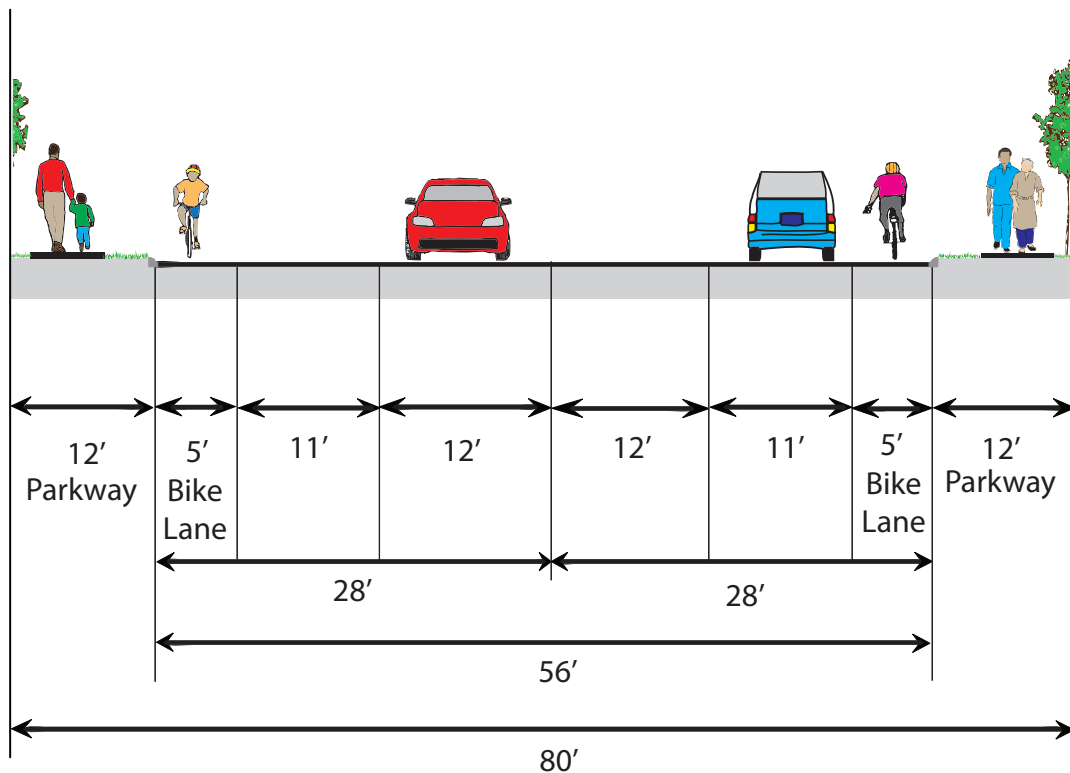
SAMPLE CROSS SECTION - MINOR ARTERIAL w/ BIKE LANE
