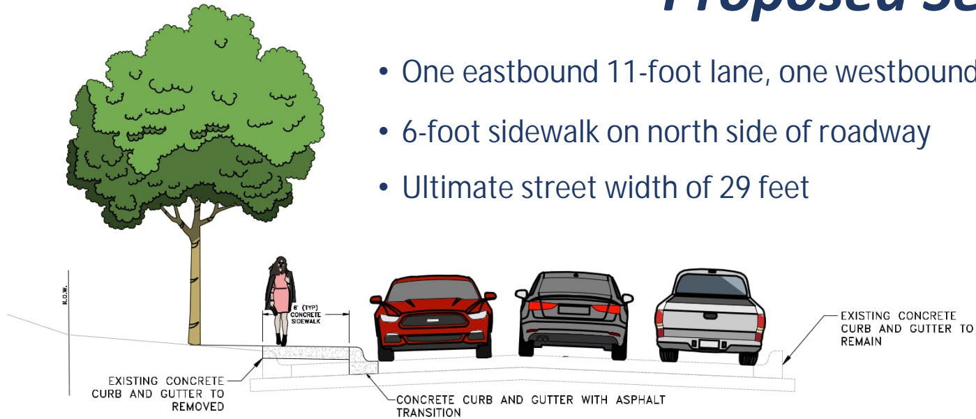
A STREET IMPROVEMENTS WITH SIDEWALK AGAINST BACK OF CURB ALONG GRAND AVENUE NOT TO SCALE
