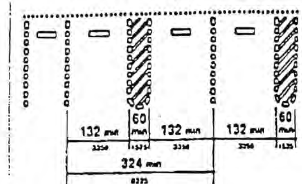
(a) Van Accessible Space at End Row
