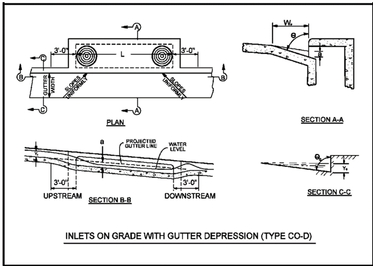
Figure 3-63.6 Type CO-D Inlet
