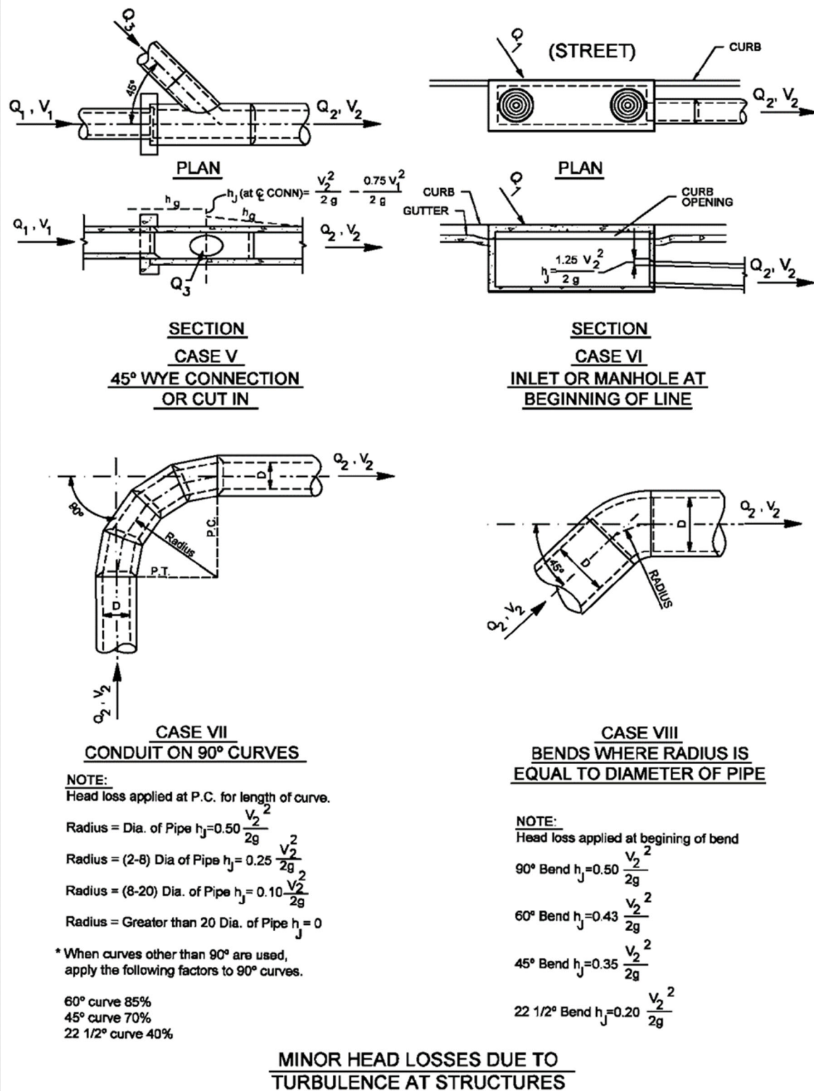
Figure 3.9 Minor Head Losses at Structures (2 of 2)
