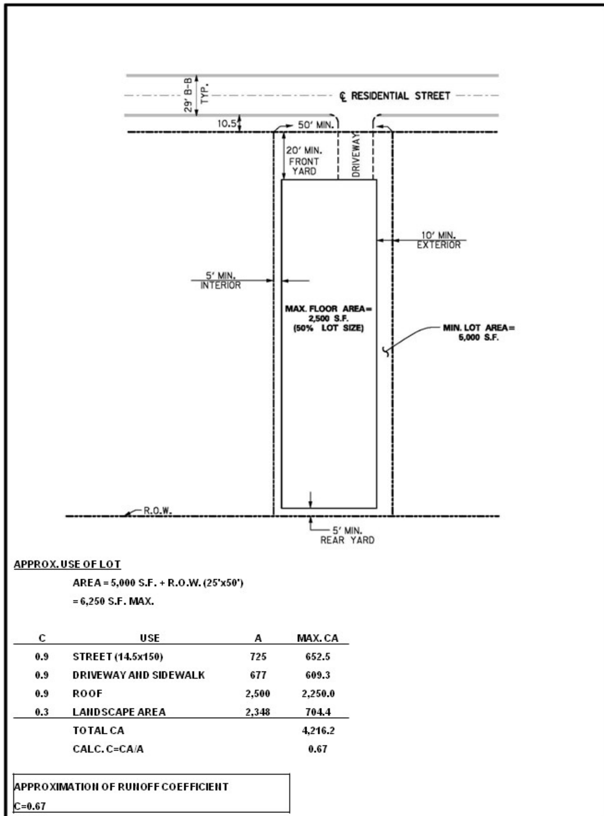
Figure 3.2 Sample Calculation Sheet for Runoff Coefficient "C"
