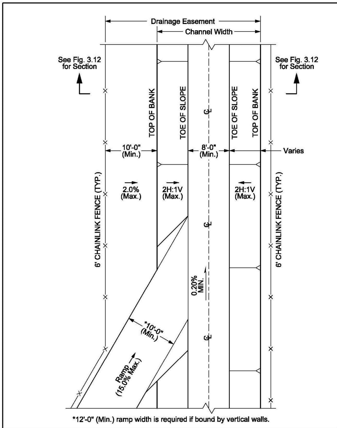
Figure 3.11 Typical 3.11 Plan -View - Trapezoidal Concrete -Lined Channel
