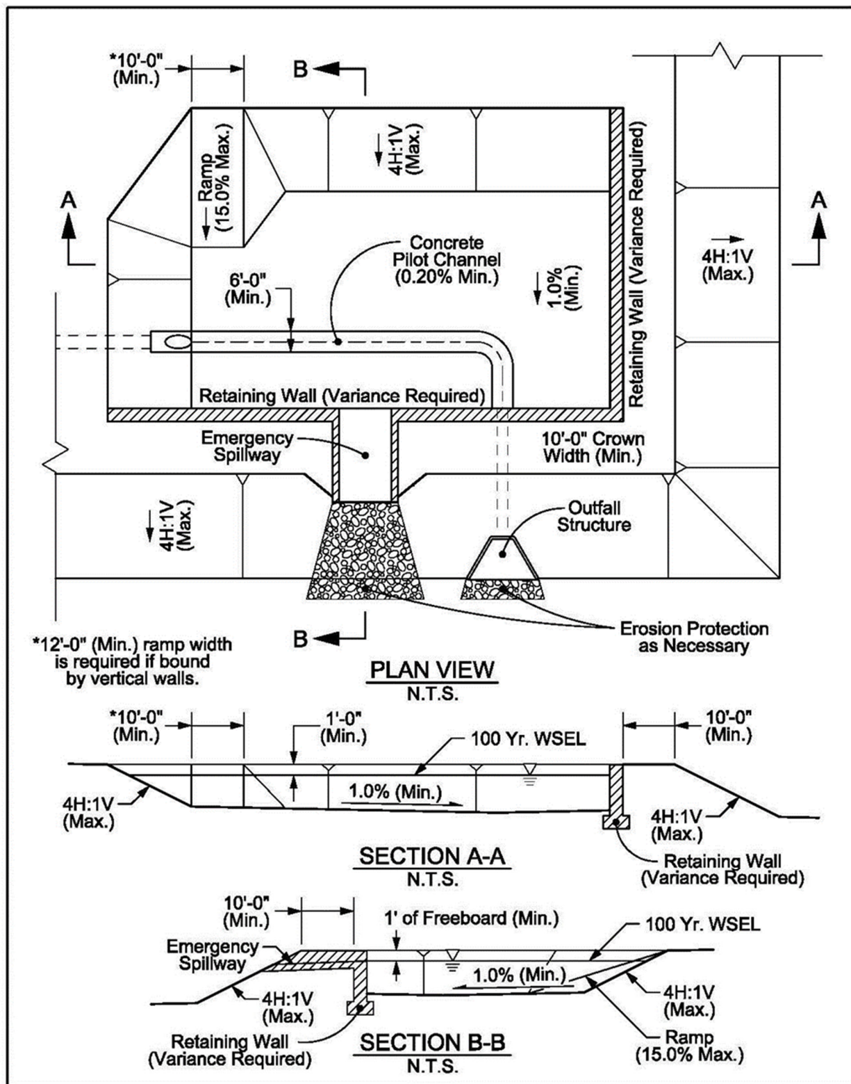
Figure 3.17 Dry Detention Pond W with Pilot Channel Schematic
