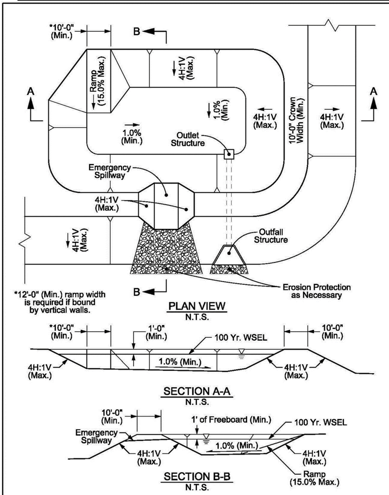
Figure 3.463.16 Dry Detention Pond Schematic
