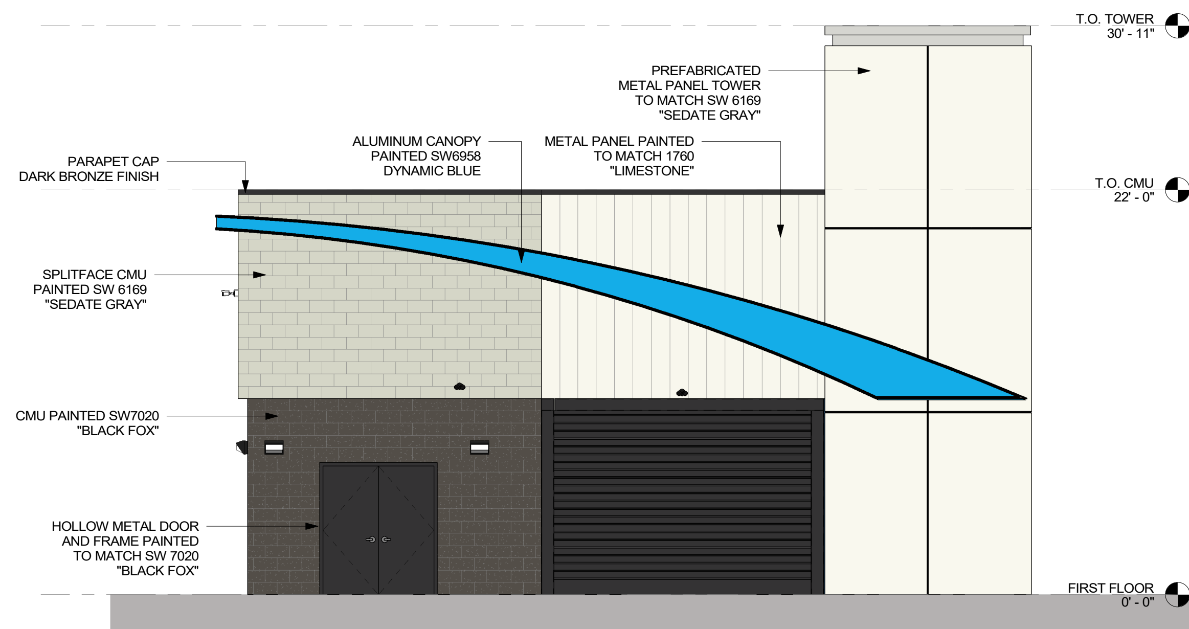
EAST ELEVATION 4 3/16" = 1'-0"
